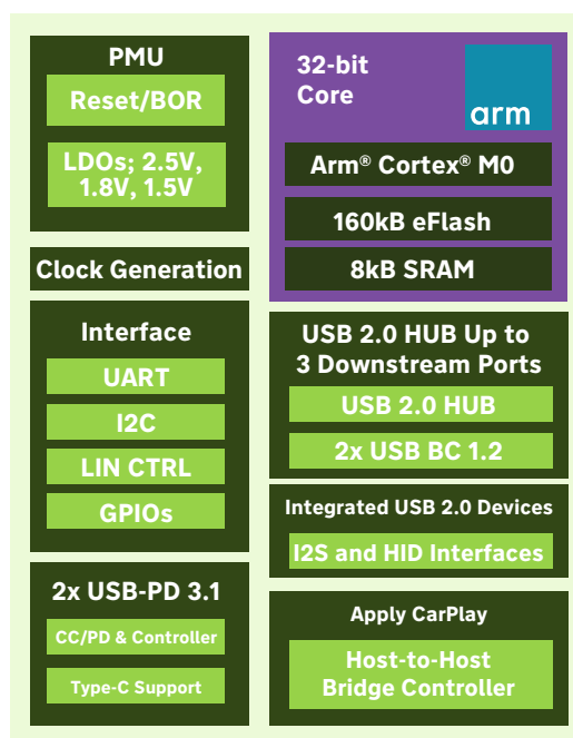
Figure 1. iND10050 Functional Diagram
